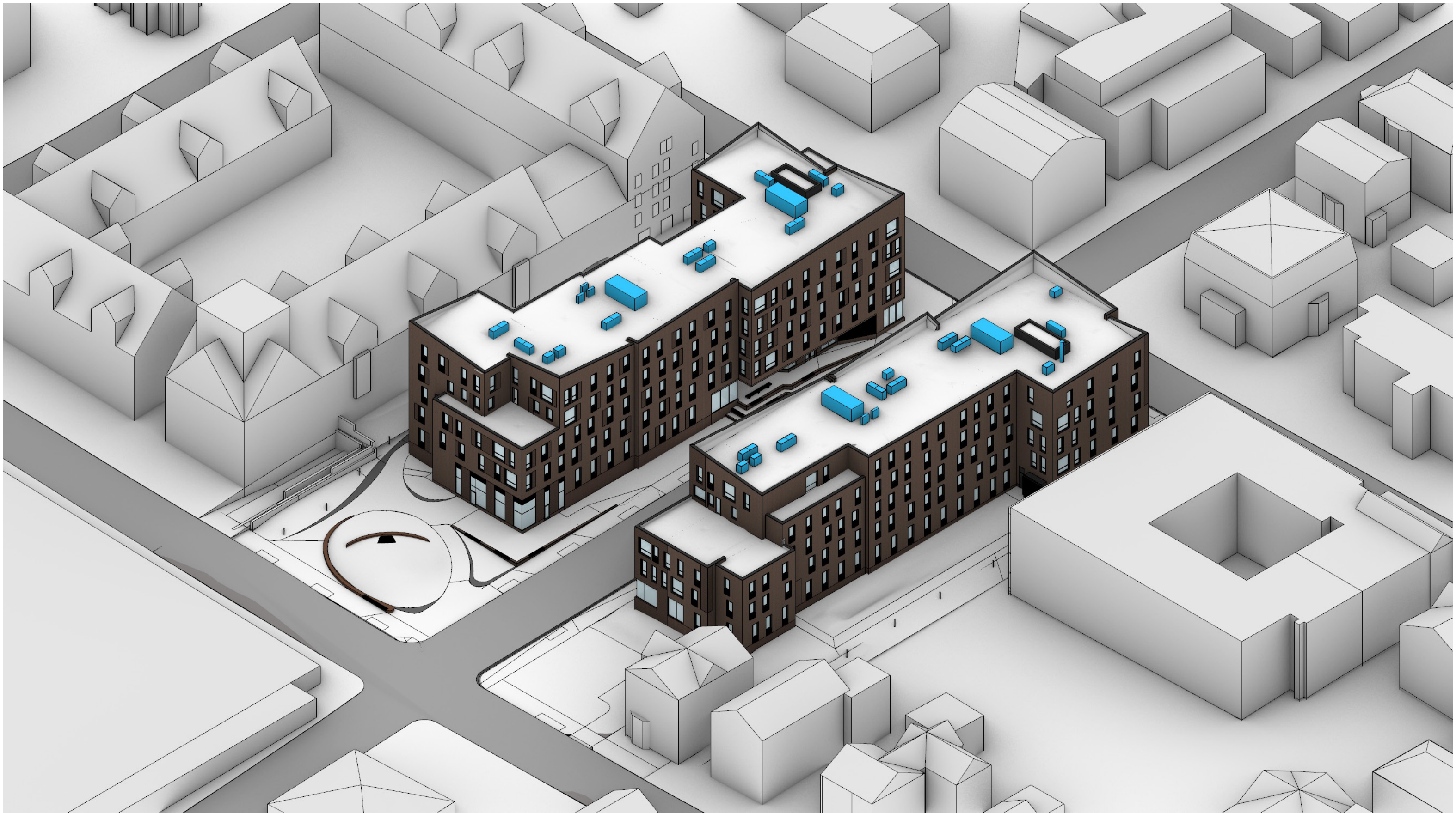
SITE AXONOMETRIC SHOWING ROOFTOP MECHANICAL EQUIPMENT IN BLUE
